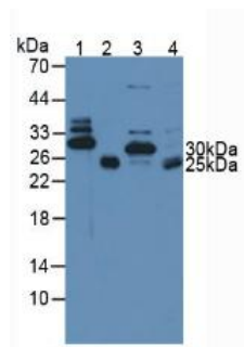
Figure. Western Blot; Sample. Lane1: Mouse Heart Tissue; Lane2: Mouse Skeletal Muscle Tissue; Lane3: Porcine Heart Tissue; Lane4: Porcine Skeletal Muscle Tissue.
